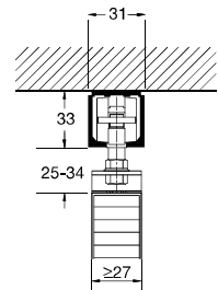
Ceiling installation Gắn trần
